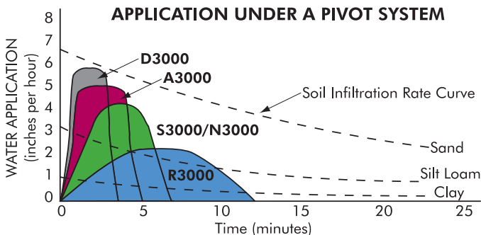
Typical Infiltration Curves combined with center pivot application rate (end of 1/4 mile system at 8 GPM/Acre and travel speed 5 fpm).
